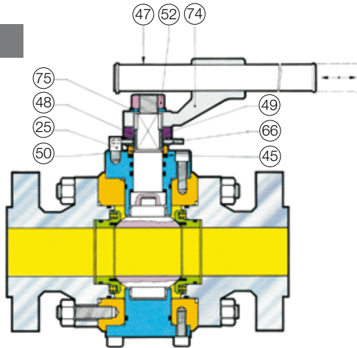
Fig. 130 Full bore
