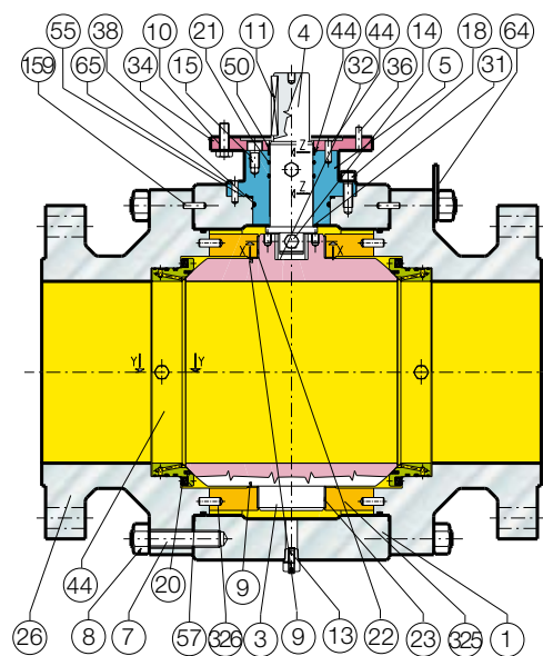
Fig. 130 Full bore
