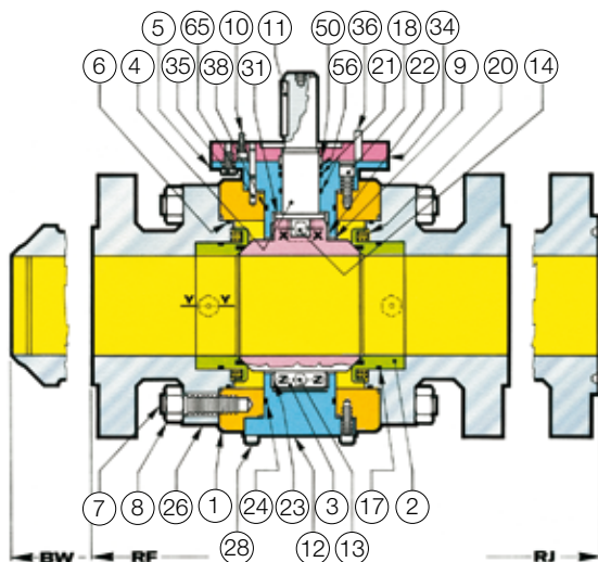
Fig. 130 Full bore
