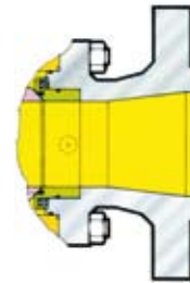
Fig. 160 Reduced bore
